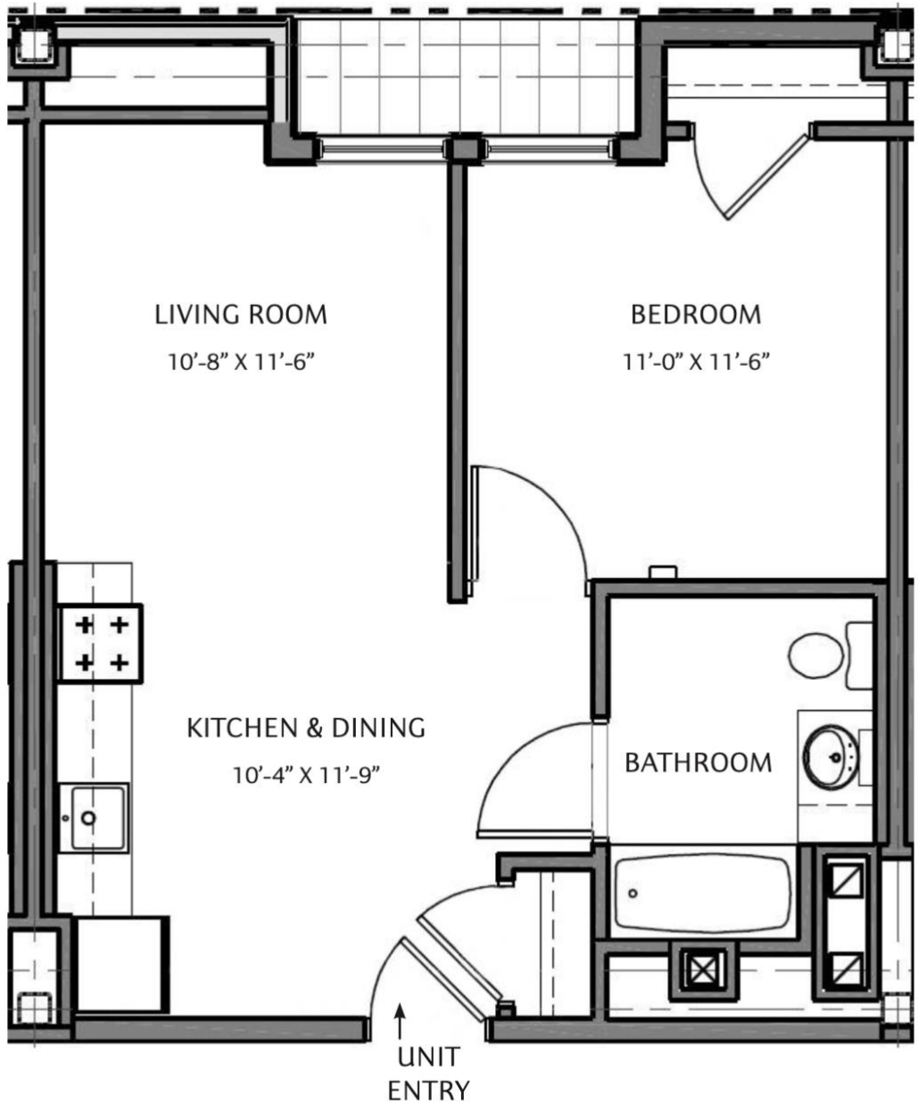
TYPE B1 UNIT - 1 BEDROOM
